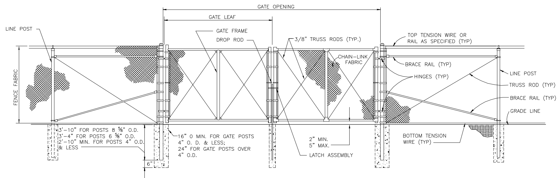
ELEVATION DOUBLE SWING GATE (TYPE FE-5 FENCE)
