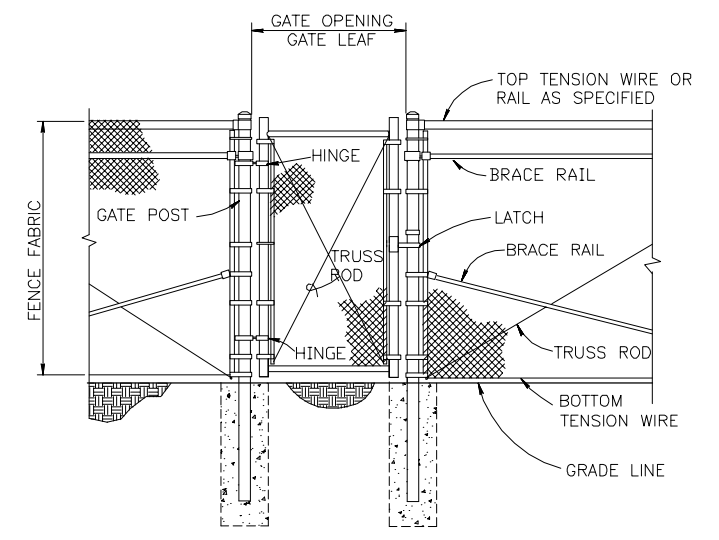
PERSONNEL GATE TYPE FE-5 FENCE
